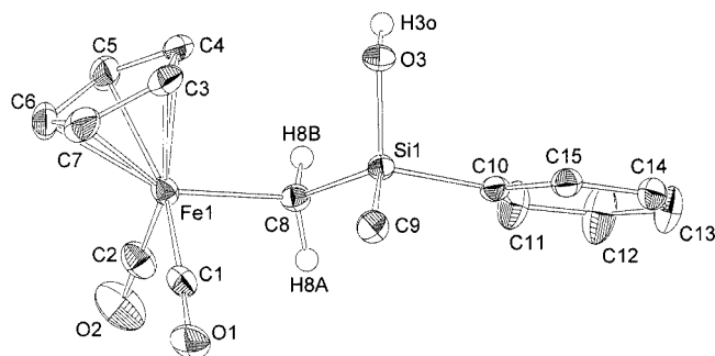
Figure 2. ORTEP view of \text{Cp}(\text{OC})_2\text{Fe}-\text{CH}_2-\text{Si}(\text{Me})(\text{Ph})\text{OH} ( 4b ); hydrogen atoms have been omitted for clarity (except for those at C8 and O3); selected bond lengths [Å] and angles [°]: Fe1–Cp(Z) 1.734(1), Fe1–C8 2.0931(18), C8–Si1 1.8464(18), Si1–O3 1.6645(13), Si1–C9 1.8598(18), Si1–C10 1.8825(19); C1–Fe1–C2 93.38(9), C1–Fe1–C8 90.98(8), C2–Fe1–C8 86.42(8), Cp(Z)–Fe1–C1 126.2(1), Cp(Z)–Fe1–C2 126.2(1), Cp(Z)–Fe1–C8 122.4(1), Fe1–C8–Si1 116.14(9), C8–Si1–O3 112.18(7), C9–Si1–O3 104.72(8), C8–Si1–C9 114.89(8), O3–Si1–C10 105.80(7); selected torsion angles [°]: Fe1–C8–Si1–O3 –67.89(10), Fe1–C8–Si1–C10 173.59(8), C1–Fe1–C8–Si1 –68.00(10), Fe1–C8–Si1–C9 51.55(12)
