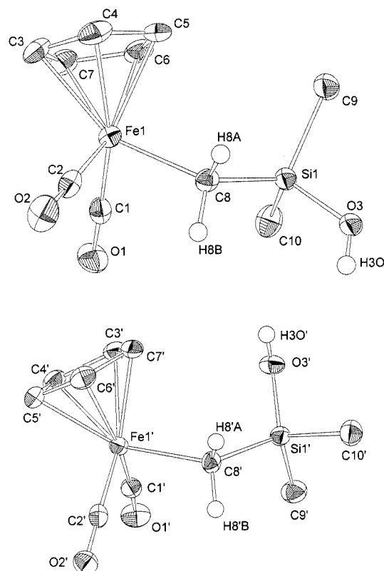
Figure 1. ORTEP view of Cp(OC)_2Fe-CH_2-SiMe_2OH ( 4a ), showing the two crystallographically independent molecules; hydrogen atoms have been omitted for clarity (except for those at C8 and O3); selected bond lengths [Å] and angles [°]: Fe1-Cp(Z) 1.728(2)/1.730(2), Fe1-C8 2.0896(16)/2.0863(17), C8-Si1 1.8451(17)/1.8508(16), Si1-O3 1.6599(13)/1.6558(13), Si1-C10 1.8596(19)/1.8686(19), Si1-C9 1.8668(17)/1.8508(18); C1-Fe1-C2 93.61(8)/93.15(7), C1-Fe1-C8 89.38(8)/92.32(8), C2-Fe1-C8 87.20(7)/85.94(7), Cp(Z)-Fe1-C1 126.8(2)/126.3(2), Cp(Z)-Fe1-C2 125.1(1)/126.5(1), Cp(Z)-Fe1-C8 123.4(1)/121.6(1), Fe1-C8-Si1 120.36(8)/120.51(8), C8-Si1-O3 108.41(7)/114.90(7), C9-Si1-O3 102.63(7)/104.03(8); selected torsion angles [°]: Fe1-C8-Si1-O3 -174.24(8)/40.09(12) , C1-Fe1-C8-Si1 70.57(11)/57.31(11), Fe1-C8-Si1-C9 71.72(12)/ -77.92(12)
