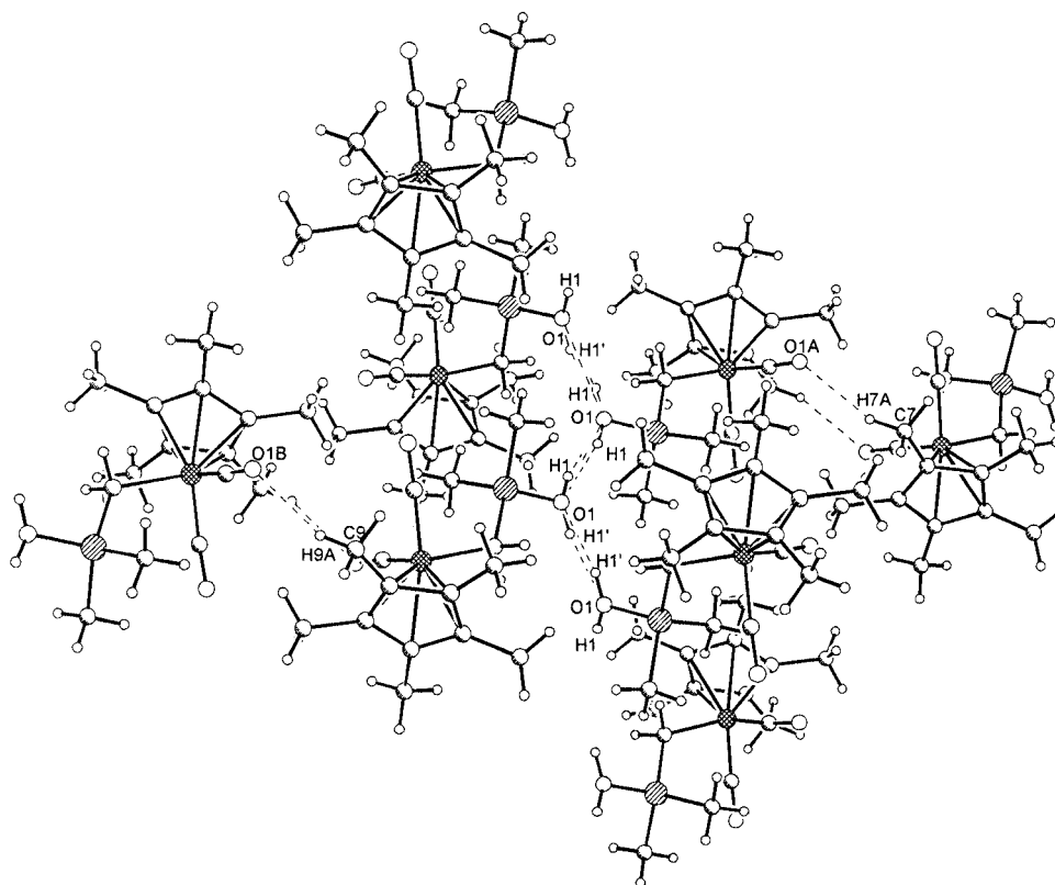
Figure 8. Connection of the chains of 4c via CH...OC interactions
