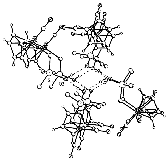
Figure 5. View inside the tube-like arrangement of the tetrameric units of 4a
