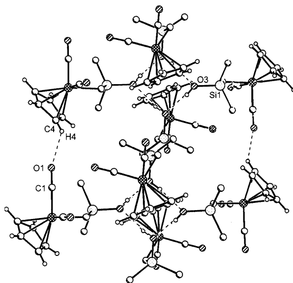
Figure 4. Ladder-type connection of 4a between the “ anti ” conformers of neighboring tetramers via \text{CH}\cdots\text{OC} bridges
