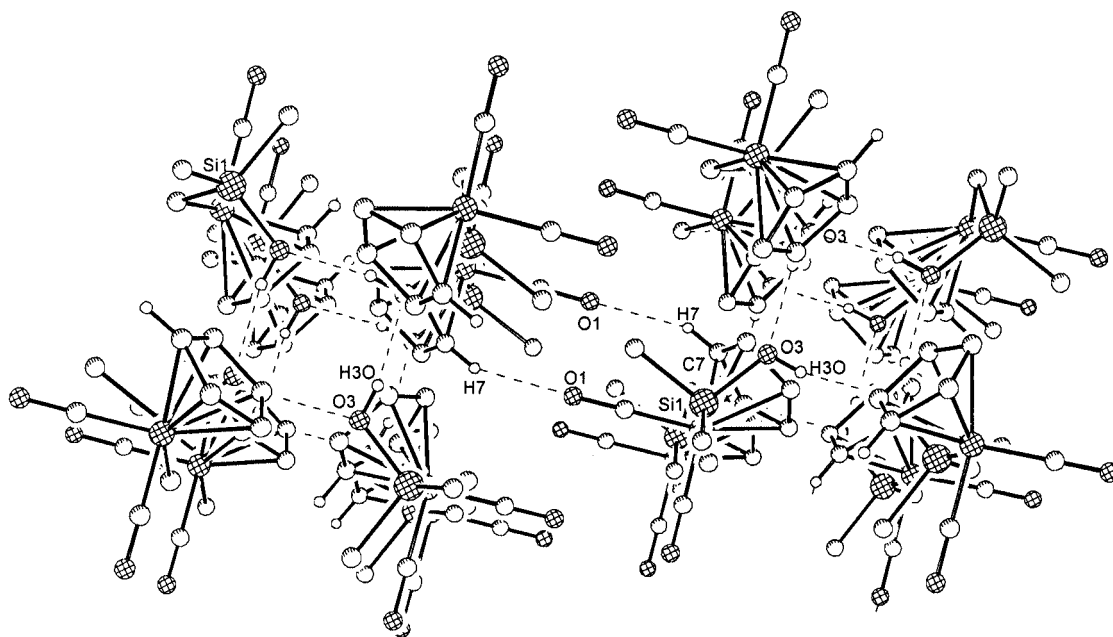
Figure 6. View inside the tube-like arrangement of the tetrameric units of 4b with connection of the tubes via CH \cdots OC bridges; hydrogen atoms (except for those involved in hydrogen bonding) as well as the phenyl carbon atoms (except for the ipso carbon atom) have been omitted for clarity
