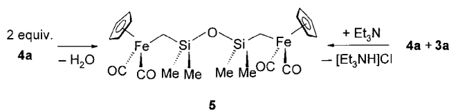
Scheme 3. Synthesis of the 1,3-bis(ferriomethyl)disiloxane 5
