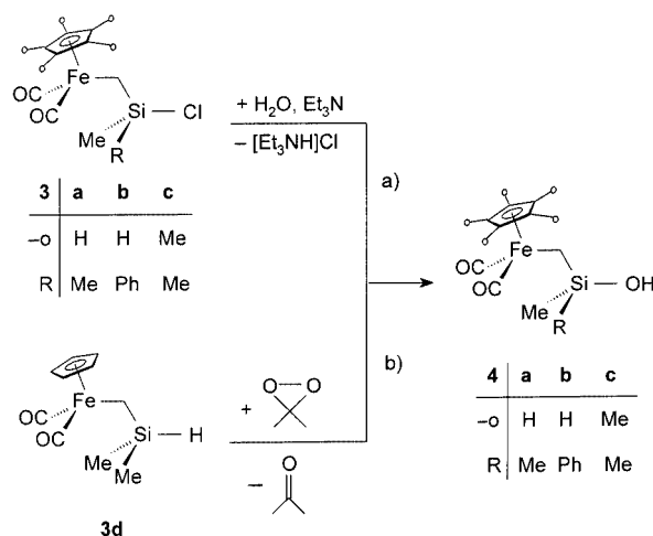
Scheme 2. Synthesis of the (ferriomethyl)silanols 4a–c by hydrolysis or oxygenation
