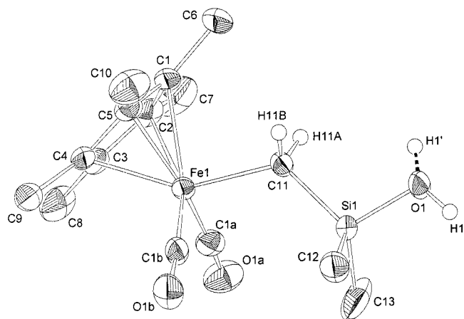
Figure 3. ORTEP view of \text{C}_5\text{Me}_5(\text{OC})_2\text{Fe}-\text{CH}_2-\text{SiMe}_2\text{OH} ( 4c ); hydrogen atoms have been omitted for clarity (except for those at C11 and O1); selected bond lengths [Å] and angles [°]: Fe1–C 5 Me 5 (Z) 1.759(2), Fe1–C11 2.0775(16), C11–Si1 1.8477(17), Si1–O1 1.6589(12), Si1–C12 1.859(2), Si1–C13 1.865(2); C1B–Fe1–C1B 97.52(9), C1B–Fe1–C11 92.17(7), C1A–Fe1–C11 92.00(8), C 5 Me 5 (Z)–Fe1–C1A 122.2(1), C 5 Me 5 (Z)–Fe1–C1B 124.1(1), C 5 Me 5 (Z)–Fe1–C11 120.7(1), Fe1–C11–Si1 124.89(9), C11–Si1–O1 106.66(7), C12–Si1–O1 106.39(8), C11–Si1–C13 114.29(10), C12–Si1–C13 107.78(13); selected torsion angles [°]: C1B–Fe1–C11–Si1 41.70(12), C1A–Fe1–C11–Si1 –55.91(12), Fe1–C11–Si1–O1 169.61(10), Fe1–C11–Si1–C12 –73.43(13), Fe1–C11–Si1–C13 50.93(16)
