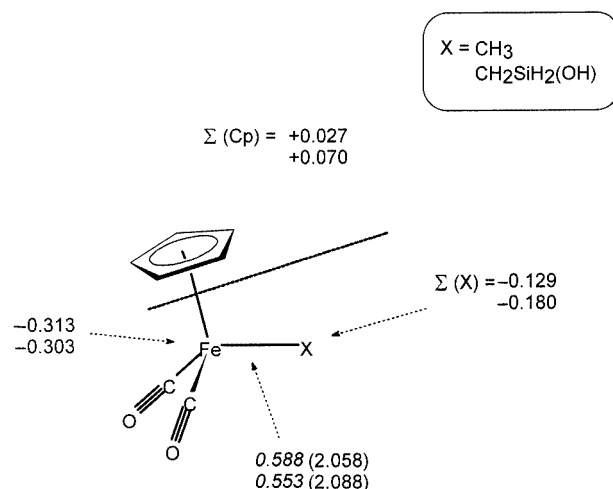
Figure 9. Population analysis of Cp(OC) _2 Fe–X (X = CH _3 , CH _2 SiH _2 OH), NBO charges and Wiberg bond indices (in italics); in parentheses are Fe–X equilibrium distances
