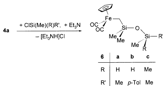
Scheme 4. Synthesis of the (ferriomethyl)disiloxanes 6a–c
