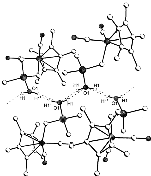
Figure 7. Chain structure of 4c via OH \cdots O bridges of the disordered SiOH proton
