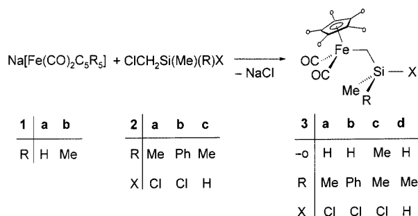
Scheme 1. Synthesis of the (ferriomethyl)silanes 3a–d
